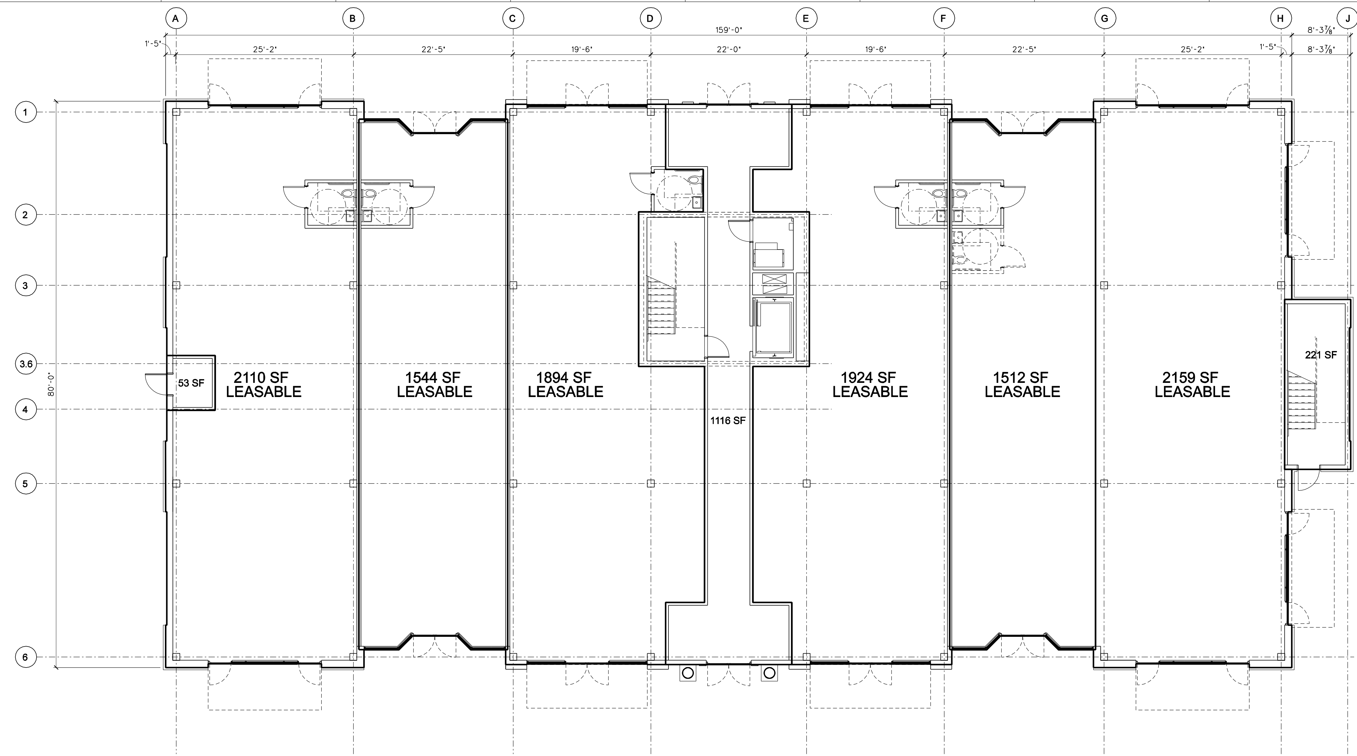
C1 FIRST FLOOR LEASING PLAN SCALE: 1/8" = 1'-0"
